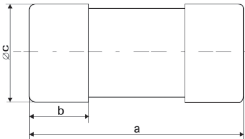
Overall dimensions of cylindrical fuse links
